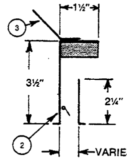
SECTION A+A WITH INTERNAL INSULATION
