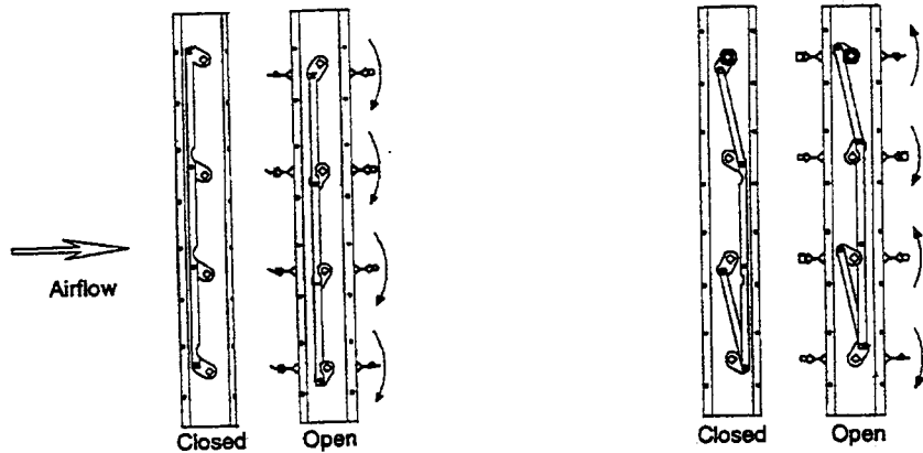
Opposed Operation Linkage
