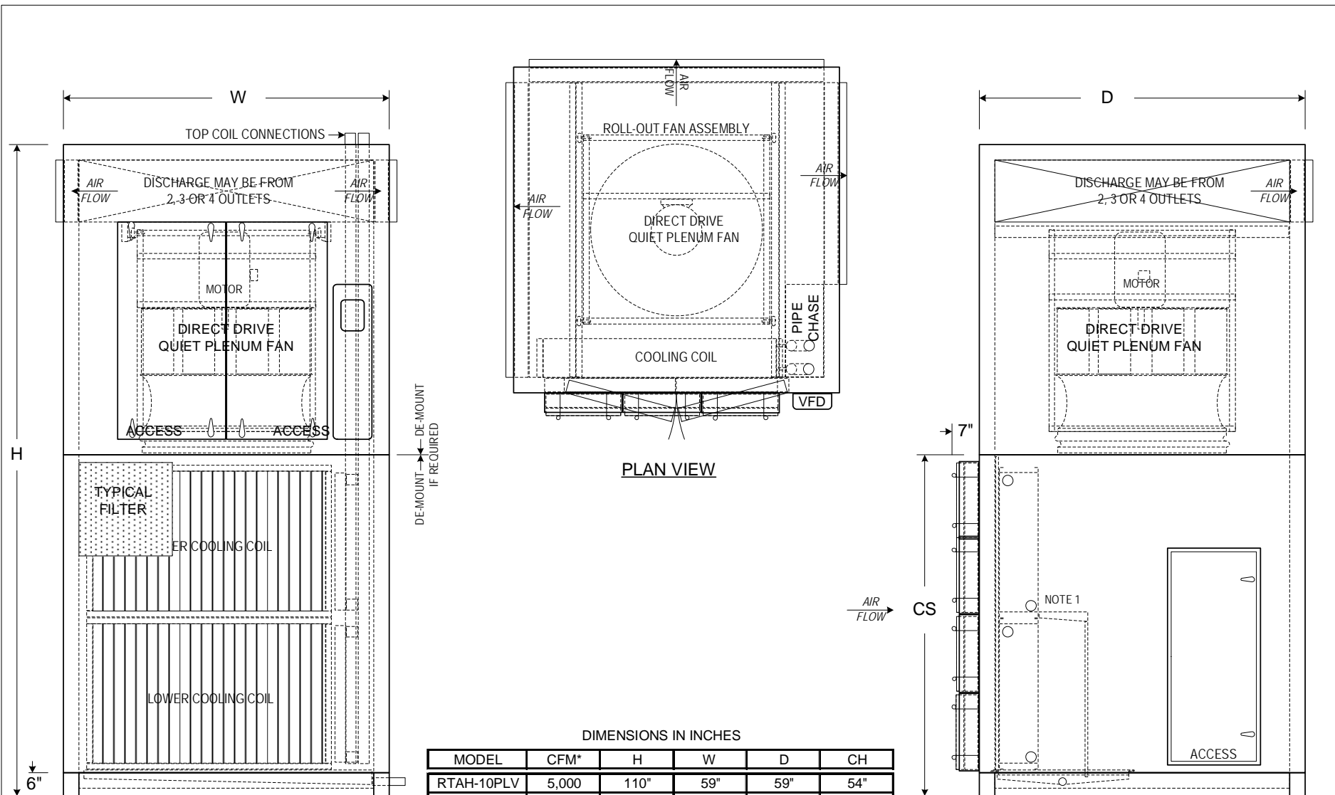
FRONT ELEVATION
